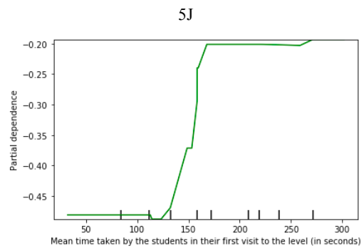
Figure 5. Partial dependence of quit probability on some of the selected features. Note that the range of y axis is different for each plot; larger ranges indicate that the feature is more predictive overall.
