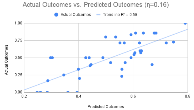
Figure 2: Actual Outcomes vs Predicted Outcomes ( \eta_k=0.16 ). When \eta_k is low, students are performing as expected from the model’s prediction.
