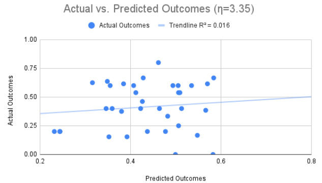
Figure 3: Actual Outcomes vs Predicted Outcomes ( \eta_k=3.35 ). When \eta_k is high, students are not performing as expected from the model’s prediction.
