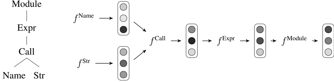
Figure 5: An illustration of the encoding process into a vector with n = 3 dimensions. We first use the Python compiler to transform the program print('Hello, _world')! into the abstract syntax tree Module(Expr(Call(Name, Str))) (left). Then, from left to right, we apply the recursive encoding scheme, where arrows represent the direction of computation and traffic light-elements represent three-dimensional vectors, where color indicates the value of the vector in that dimension.
