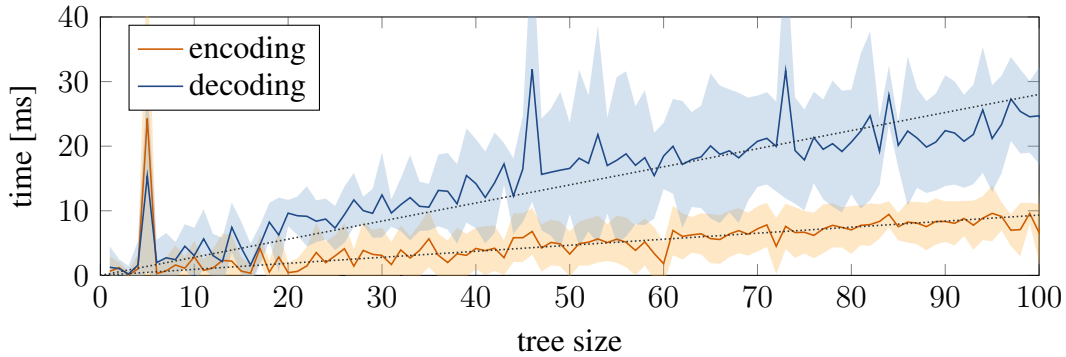
Figure 9: The time needed for encoding (orange) and decoding (blue) trees of different sizes for the DT chatbot course. The thick lines mark the means whereas shaded regions indicate one standard deviation. The dotted lines indicate the best linear fit.
