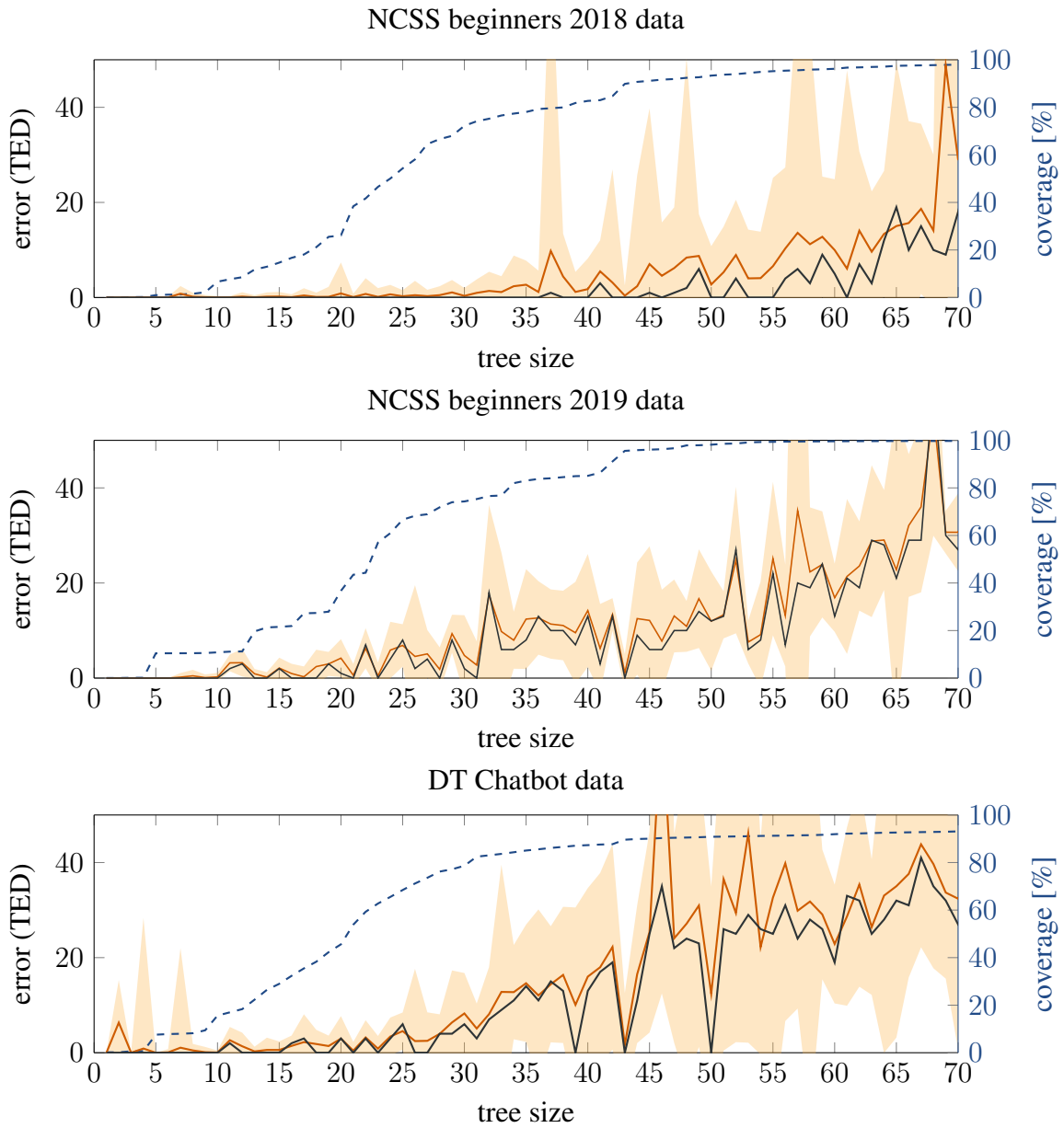
Figure 8: The autoencoding error as measured by the tree edit distance for the NCSS 2018 beginners challenge (top), NCSS 2019 beginner challenge (middle) and DT chatbot course (bottom). The error is plotted here versus tree size. The orange line marks the mean, the black line the median error. The orange region is the standard deviation around the man. Additionally, the blue line indicates how many trees in the dataset have a size up to x .
