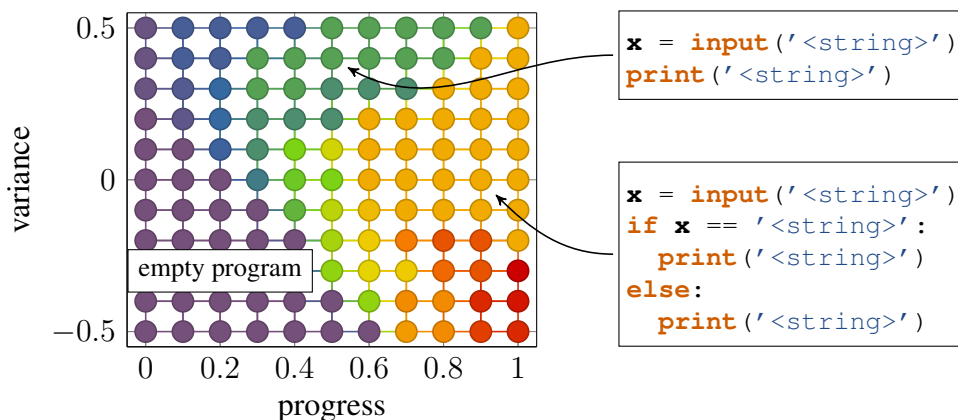
Figure 12: A linear interpolation between the empty program at (0, 0) and the correct solution at (1, 0) as well as along the axis of biggest variation. Color indicates the tree that the grid point decodes to. The three most common trees are shown in the boxes.
